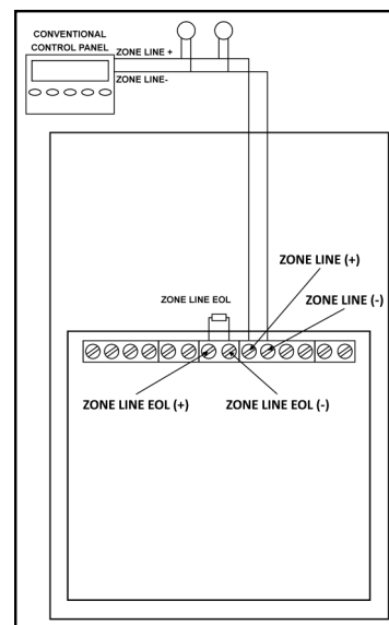
Picture 10 - Conventional line wiring (zone line EOL resistor inside of the device)
