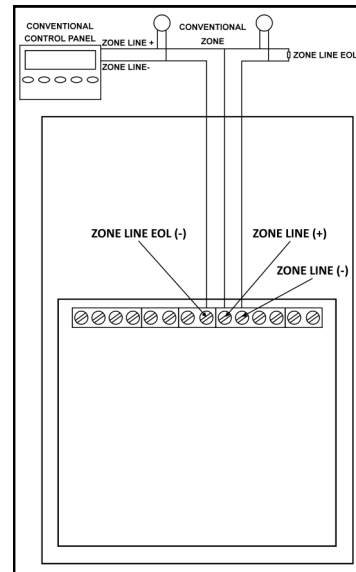
Picture 9 - Conventional line wiring (zone line EOL resistor outside of the device)
